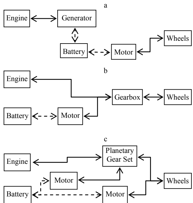
Fig. 2. Hybrid configurations: a – series; b – parallel; c – complex configurations
