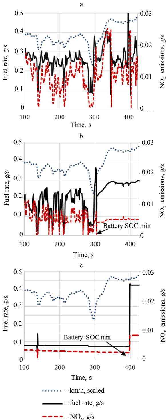
Fig. 9. Fuel rate against NO x emissions: a – conventional; b – parallel; c – series
