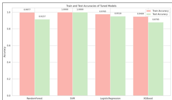
Figure 2. Performance metrics of models for cognitive domain.
