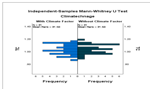
Figure A3. TC distribution with and without climate impact
