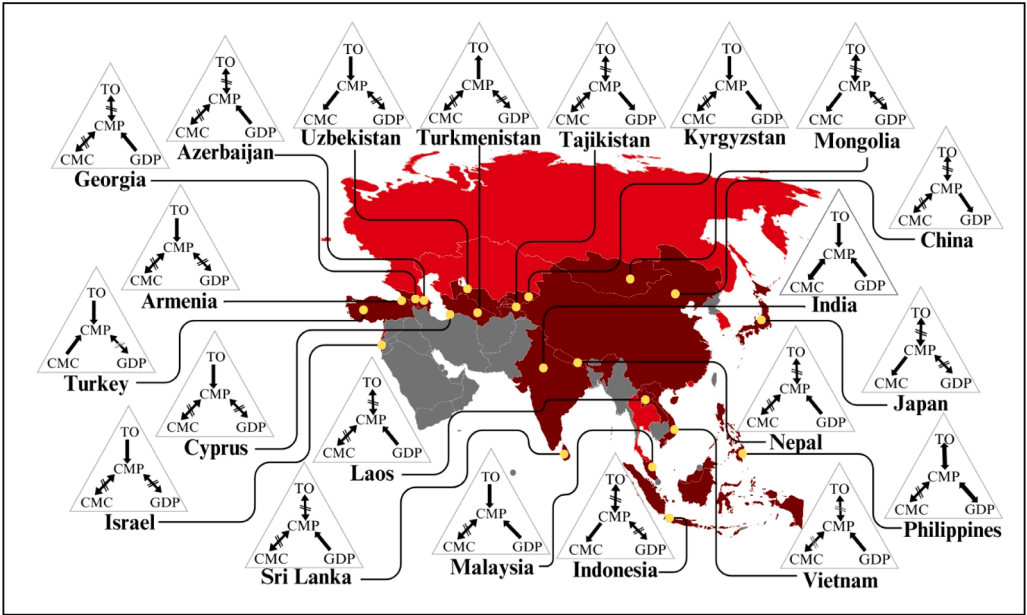
Fig. 6. Granger causality results for Asian countries. Note: The triangle shapes in the figure represent the causal flows from chicken meat production (CMP) to chicken meat consumption (CMC), GDP, and trade openness (TO), respectively. Source: Authors' illustrations-based Granger analysis results.
