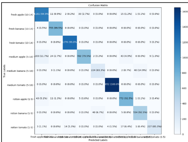
Figure 10: Confusion Matrix for freshness and shelf-life prediction
