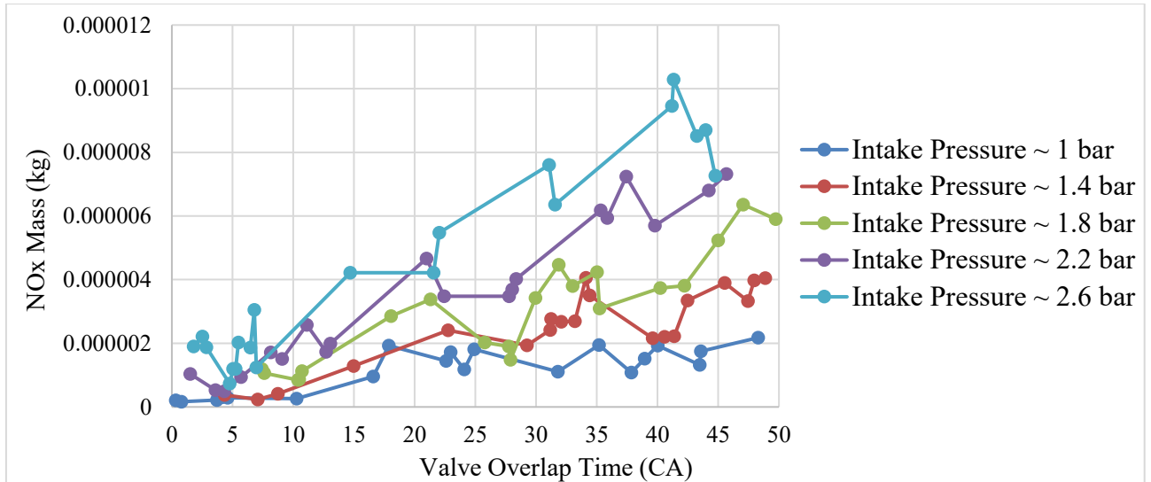
Figure 6: Effect of VOT on NO x emissions at various intake pressures
